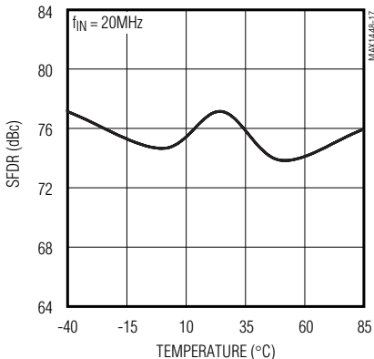
SPURIOUS-FREE DYNAMIC RANGE vs. TEMPERATURE ( f_{IN} = 20MHz )
