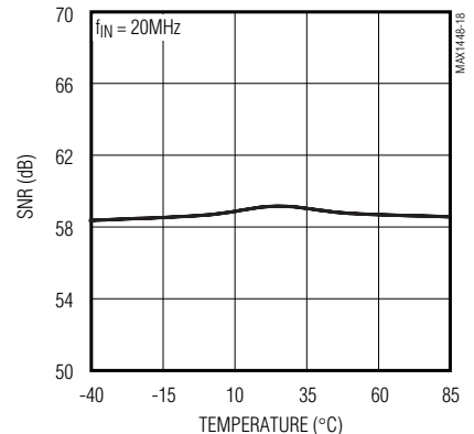
SIGNAL-TO-NOISE RATIO vs. TEMPERATURE ( f_{IN} = 20MHz )
